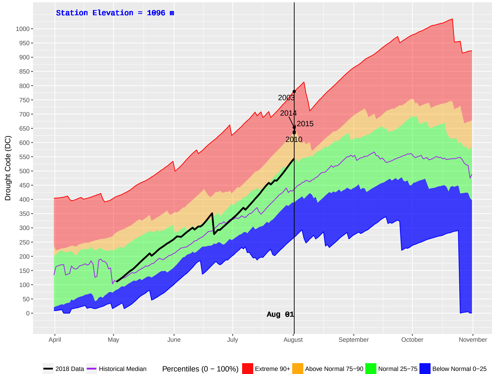
ANAHIM LAKE HUB (213) : Historical (1981–2016) and Current (2018) Daily Drought Code (DC)
