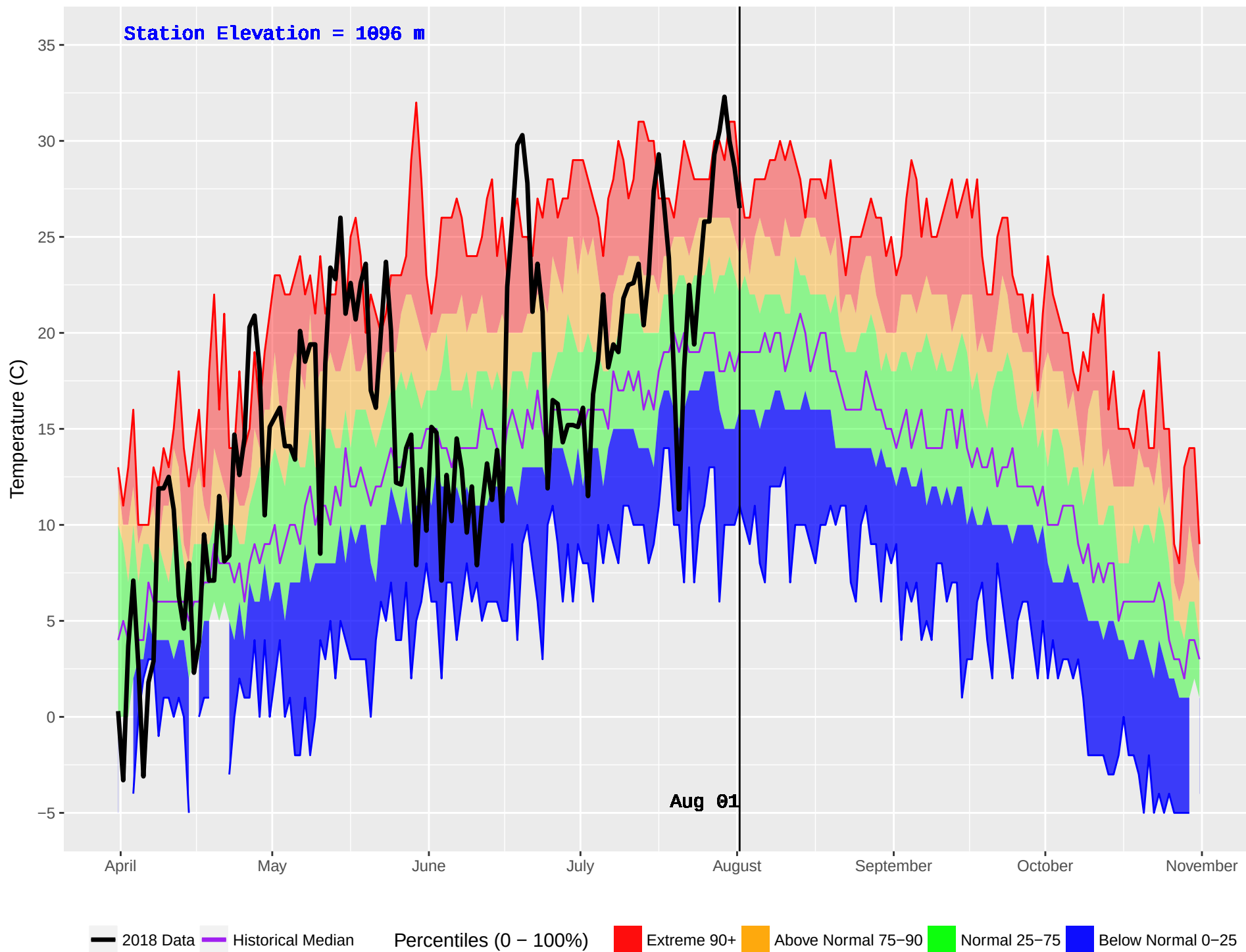
ANAHIM LAKE HUB (213) : Historical (1981–2016) and Current (2018) Daily Temperature
