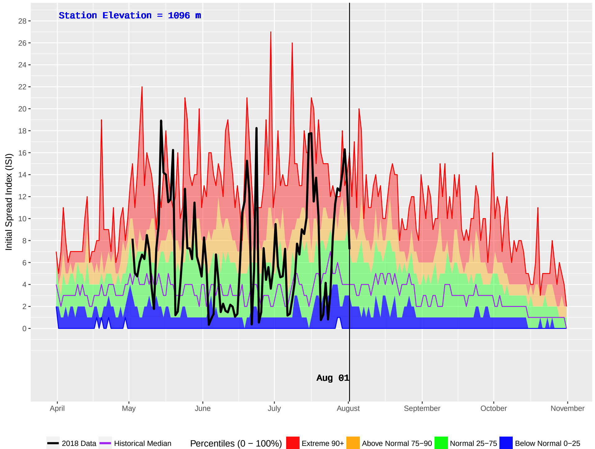
ANAHIM LAKE HUB (213) : Historical (1981–2016) and Current (2018) Daily Initial Spread Index (ISI)
