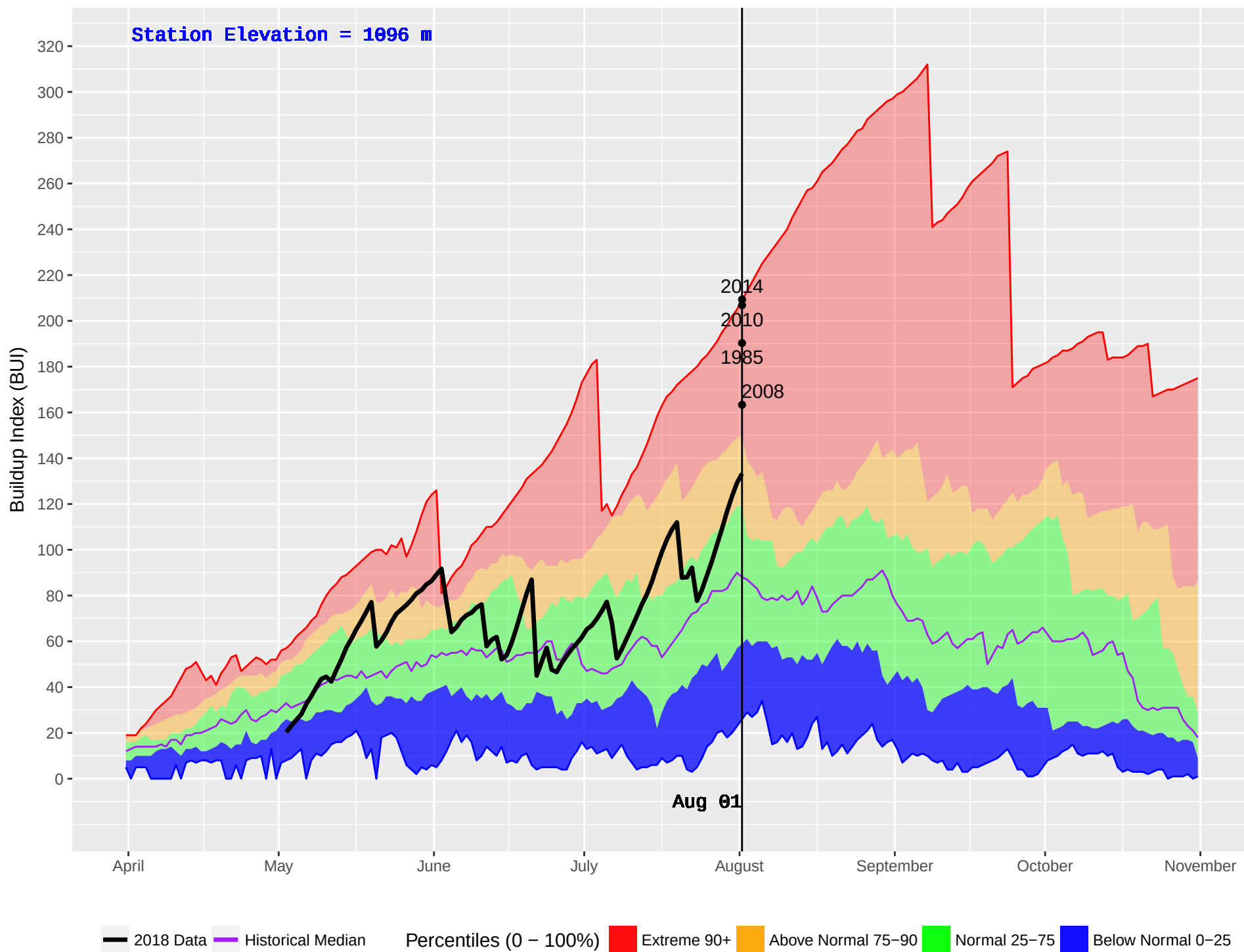
ANAHIM LAKE HUB (213) : Historical (1981–2016) and Current (2018) Daily Buildup Index (BUI)
