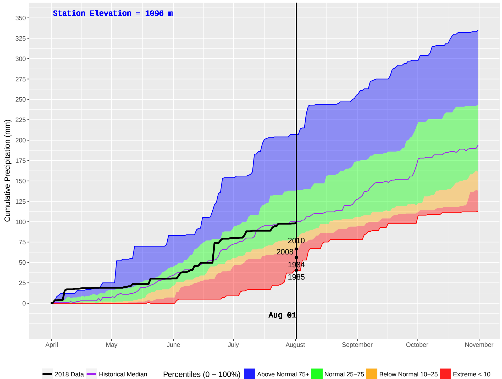
ANAHIM LAKE HUB (213) : Historical (1981–2016) and Current (2018) Daily Cumulative Precipitation
